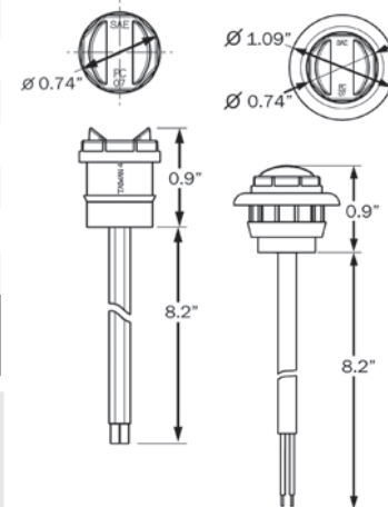
HOLE CUT-OUT: 0.75"
