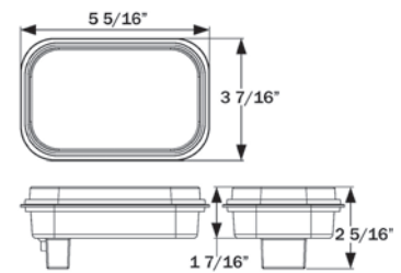
HOLE CUT-OUT: 5.462" x 3.562" (1" R)
