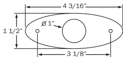
HOLE CUT-OUT: 1"
