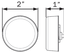
HOLE CUT-OUT: 2.313"
