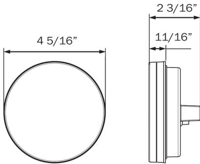
HOLE CUT-OUT: 4.5"
