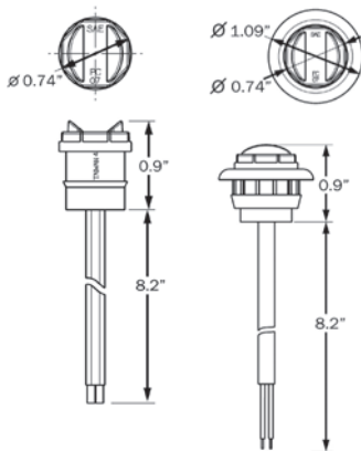
HOLE CUT-OUT: 0.75"
