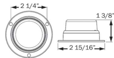
SURFACE MOUNT
