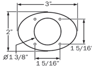
HOLE CUT-OUT: 1.375"
