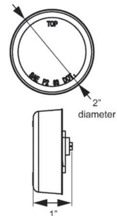
HOLE CUT-OUT: 2.313"
