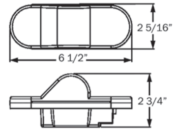
HOLE CUT-OUT: 6.85" X 2.5" (1.25" R)
