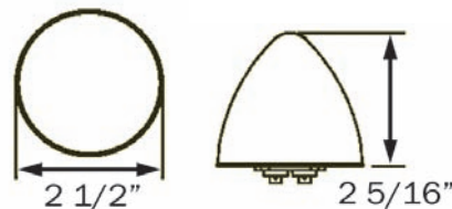
MCL23 SERIES HOLE CUT-OUT: 2.75"
