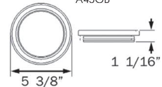
HOLE CUT-OUT: 4.5"
