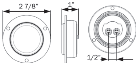
HOLE CUT-OUT: 2.313"
