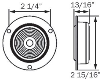
MC52 Black Flange
