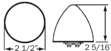
MC27 SERIES HOLE CUT-OUT: 2.75"
