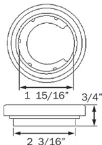
HOLE CUT-OUT: 2.313"
