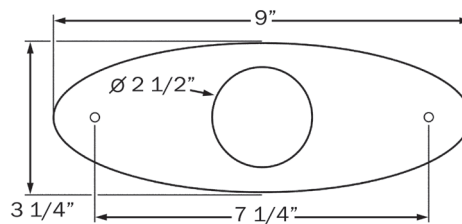
HOLE CUT-OUT: 2.5"
