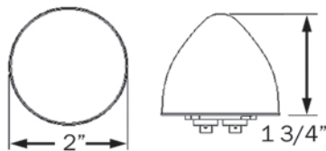
MC25 SERIES HOLE CUT-OUT: 2.313"
