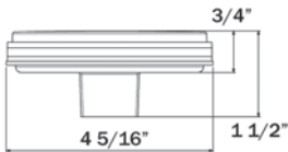
HOLE CUT-OUT: 4.5"
