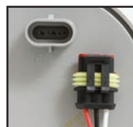
Weathertight connection
