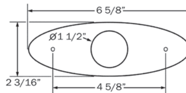
HOLE CUT-OUT: 1.5"
