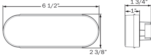
HOLE CUT-OUT: 6.85" x 2.52" (1.26" R)
