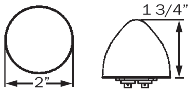
MCL21 SERIES HOLE CUT-OUT: 2.313"
