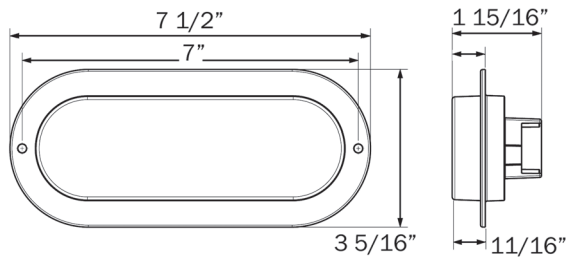
HOLE CUT-OUT: 6.85" X 2.5" (1.25" R)
