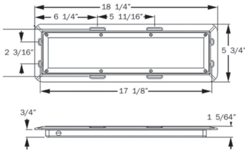
ILL08/28/10 SERIES DIMENSIONS
